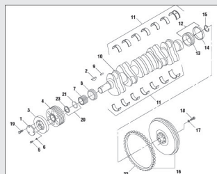
Assembly Drawing
